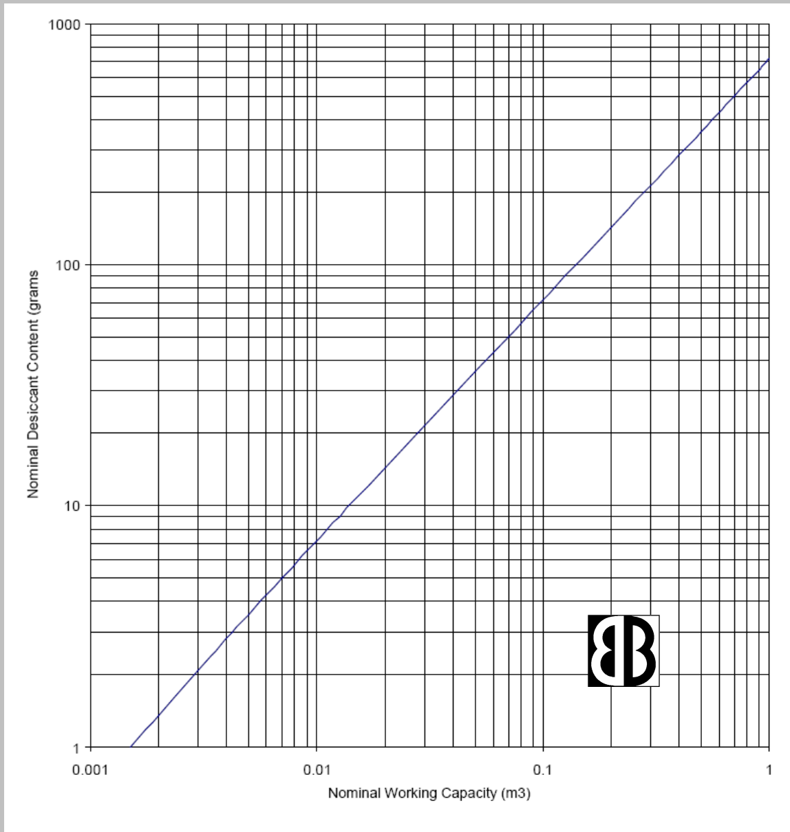
Desiccant content chart for working capacities up to 1m 3
